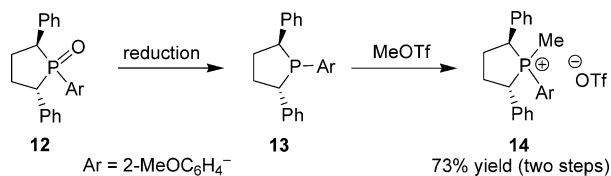
Scheme 5. Synthesis of 1-aryl-1-alkylphospholanium salt 14 .
