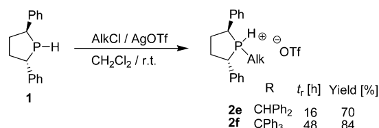
Scheme 4. Alkylation of phospholane 1 with alkyl chlorides.
