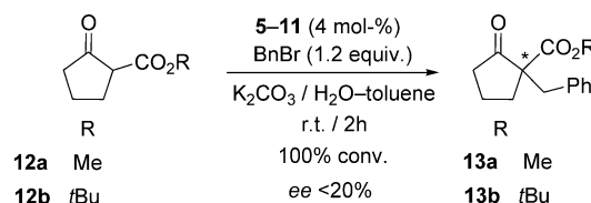
Scheme 6. Phase-transfer alkylation.
