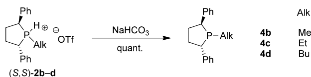
Scheme 3. Deprotection of phospholanium salts 2b–d .
